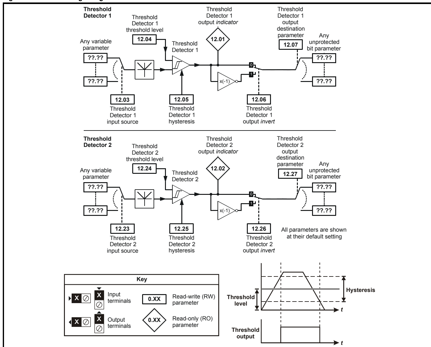
Figure 5-11 Menu 12 logic diagram
